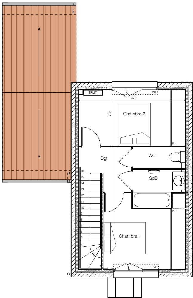
Plan R+1
