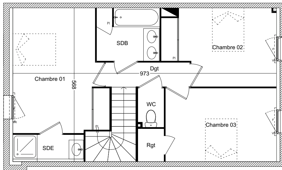
Plan R+1
